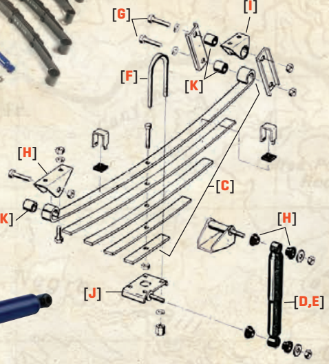
1972-75 Suspension
